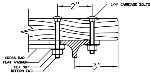
SECTION - LEG, BRACE & WOOD
