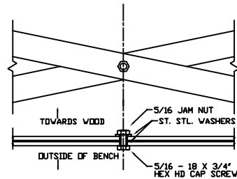
DETAIL OF BACK BRACE
